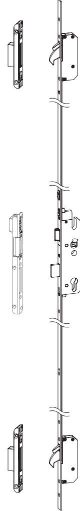
AV3 – AUTOMATIC LOCKING SYSTEM WITH MAGNETIC TRIGGER AND DAY LATCH FUNCTION
